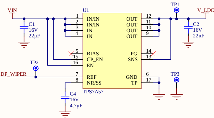
Variable Output LDO
