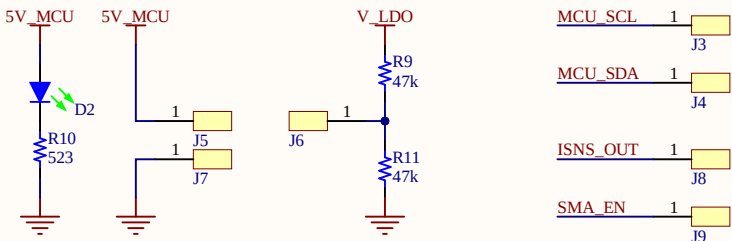
MCU Connections
